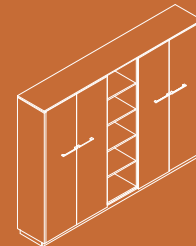
X5119 2496x421x1871
